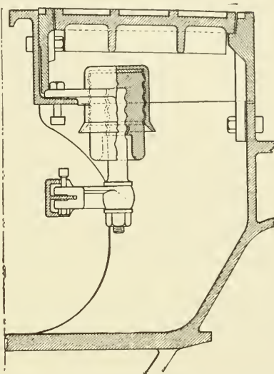
Fig. 242. Section of Underground Conduit Showing Handhole
